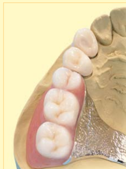
Vario-Soft 3 matrix housing
